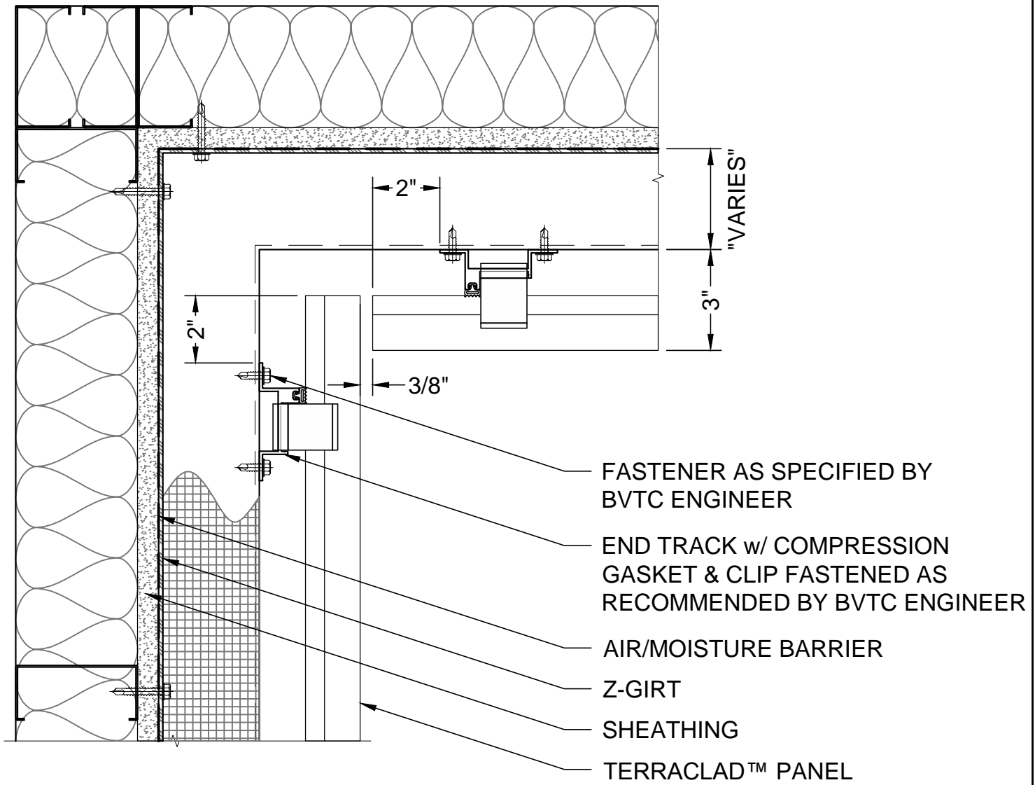
1 PLAN DETAIL INSIDE CORNER w/ 3/8" JOINT Scale: 3" = 1'-0"
