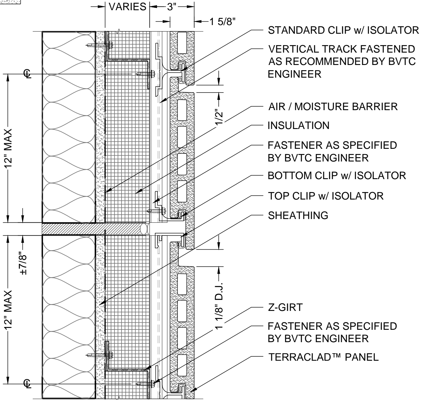
SECTION DETAIL PANEL AT EXPANSION JOINT 1 Scale: 3" = 1'-0"
