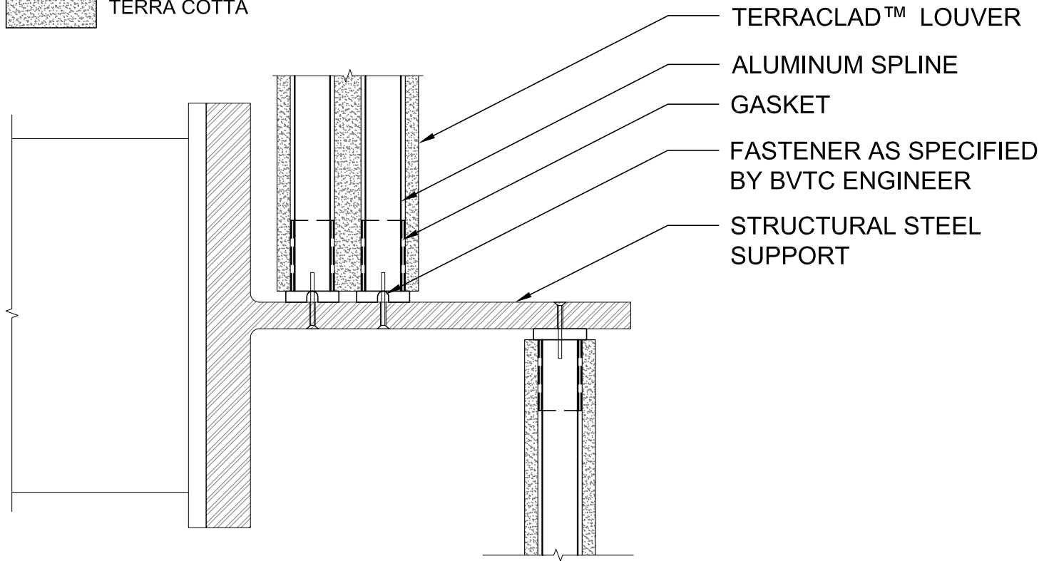
2 SECTION DETAIL LOUVER SUPPORT SYSTEM Scale: 3" = 1'-0"
