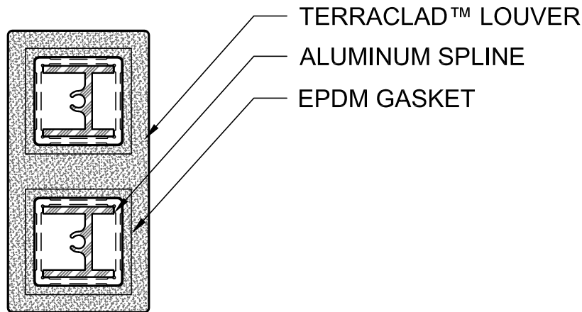
1 SECTION DETAIL 2" x 4" LOUVER Scale: 6" = 1'-0"
