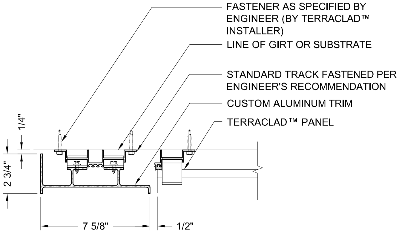
SECTION DETAIL 8" VERTICAL TRIM
