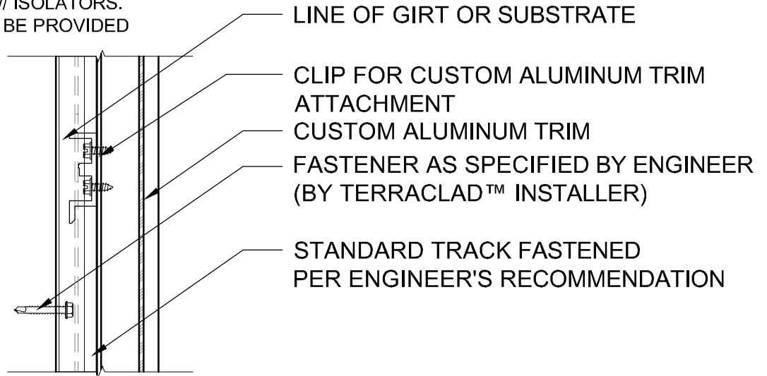
SECTION DETAIL 8" VERTICAL TRIM
